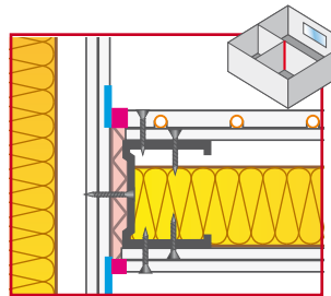
▲ T-connection, double-layer planking
